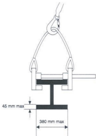
Rollclamp M
