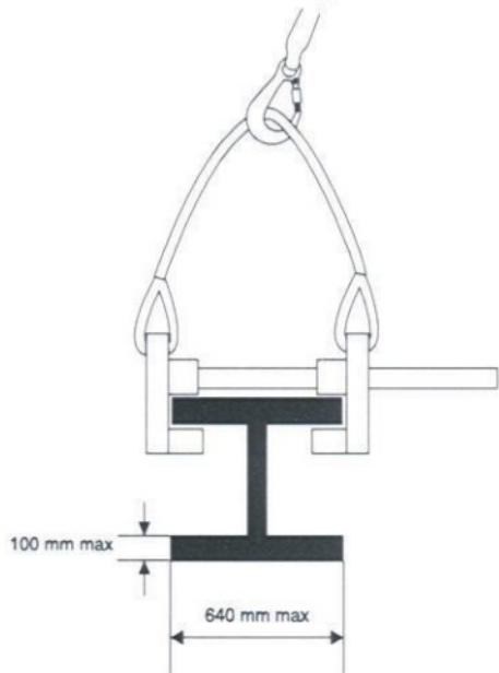
Rollclamp L
